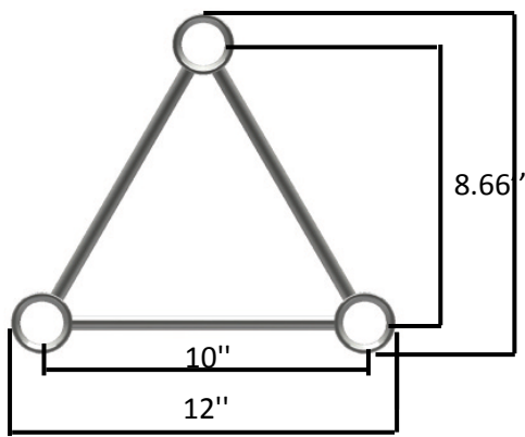
TRUSS END VIEW
